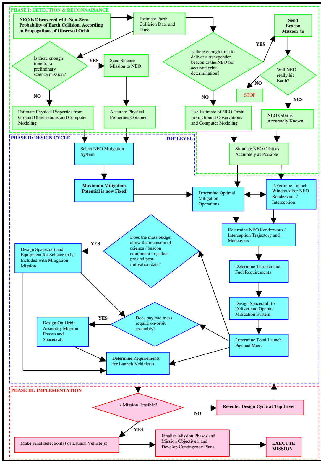
Figure 3: NEO mitigation mission planning flowchart
