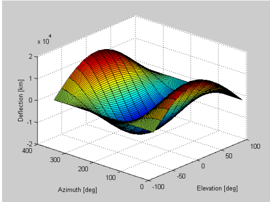
Figure 8: Deflection solution space surface in azimuth and elevation. The maximum deflection is achieved at an elevation angle of zero.
