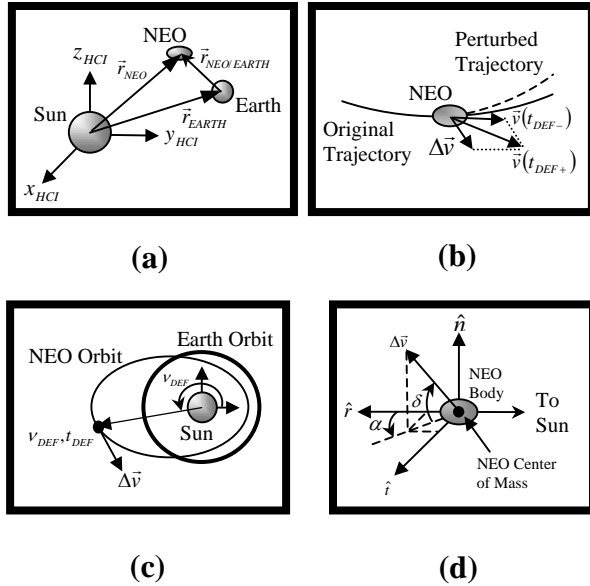
Figure 6: (a) The relative geometry between the NEO and Earth in the heliocentric inertial (HCI) frame. (b) The geometry of a velocity perturbation being applied to the NEO's inertial velocity vector. (c) An illustration of a time of deflection and corresponding true anomaly of the deflection point on the NEO's orbit. (d) The geometry of the deflection velocity change vector in the NEO's Radial-Transverse-Normal (RTN) reference frame in terms of spherical coordinate angles \alpha and \delta , termed the azimuth and elevation, respectively.
