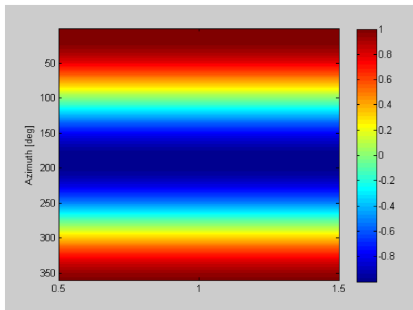
Figure 10: Spectral plot of normalized deflection as a function of azimuth angle, where a value of 1 indicates maximum deflection.
