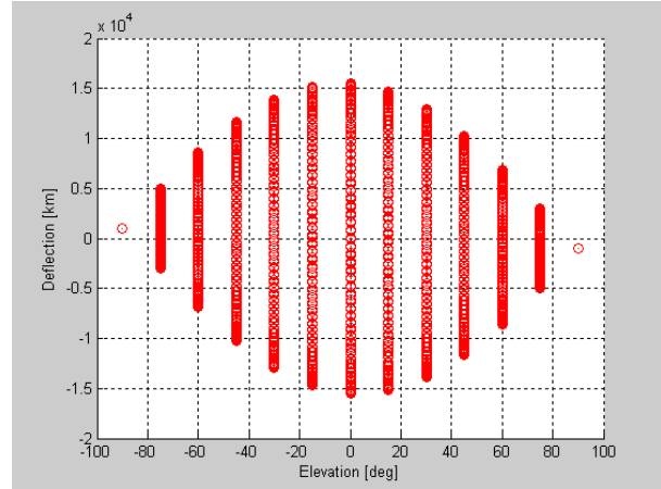
Figure 11: Deflection as a function of elevation showing lines of constant azimuth.
