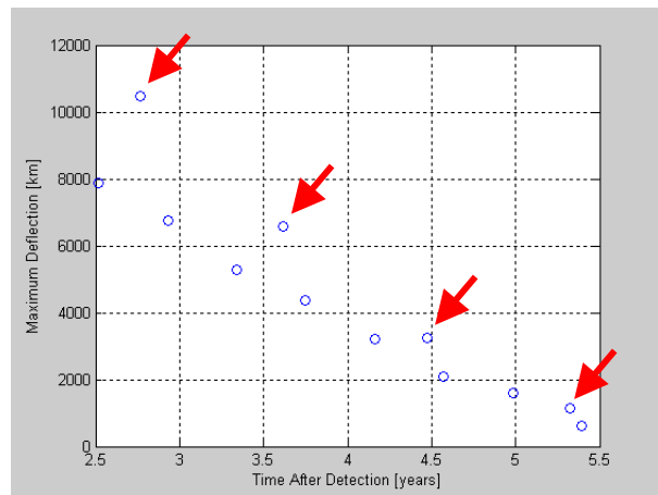
Figure 7: Deflection as a function of time for optimally oriented impulsive velocity change vectors. Times for which the NEO is at perihelion are marked with red arrows.
