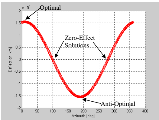
Figure 9: Deflection as a function of azimuth for a constant elevation angle of zero.
