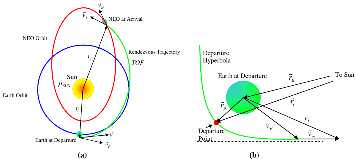
Figure 1. (a) Geometry for Lambert targeting between the Earth and a NEO and (b) Earth departure geometry.
