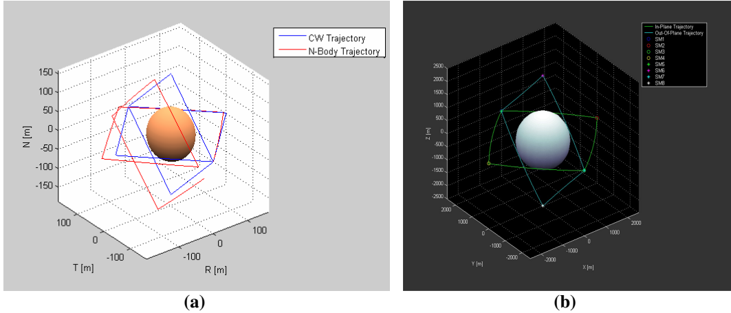
Figure 10. Waypoint-based relative motion trajectories about a NEO (a) showing both linearized dynamics motion and non-linear dynamics motion including NEO gravity 7 and (b) showing only linearized motion and waypoints 8 .
