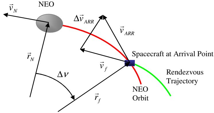
Figure 2. Geometry at NEO arrival.
