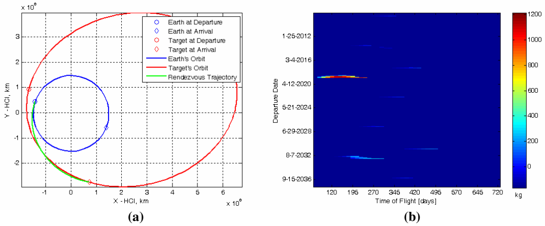
Figure 5. (a) Maximum Payload Mass Rendezvous with Asteroid 1986 DA and (b) Maximum Payload Mass as a Function of Departure Date and Time of Flight
