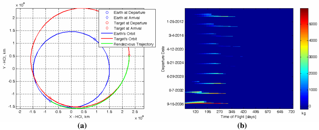
Figure 8. (a) Maximum Payload Mass Rendezvous with Asteroid Itokawa and (b) Maximum Payload Mass as a Function of Departure Date and Time of Flight
