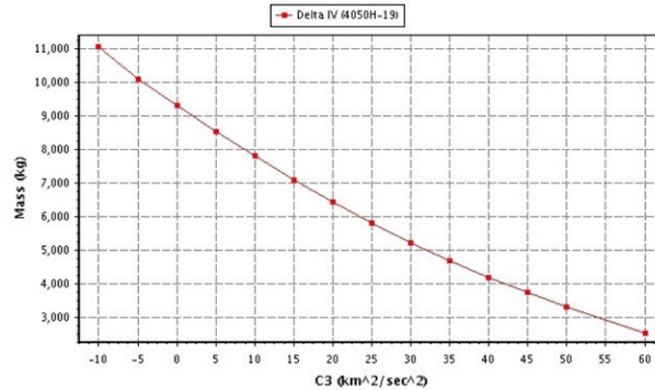
Figure 4. Launch payload mass performance for the Boeing Delta-IV Heavy † .
