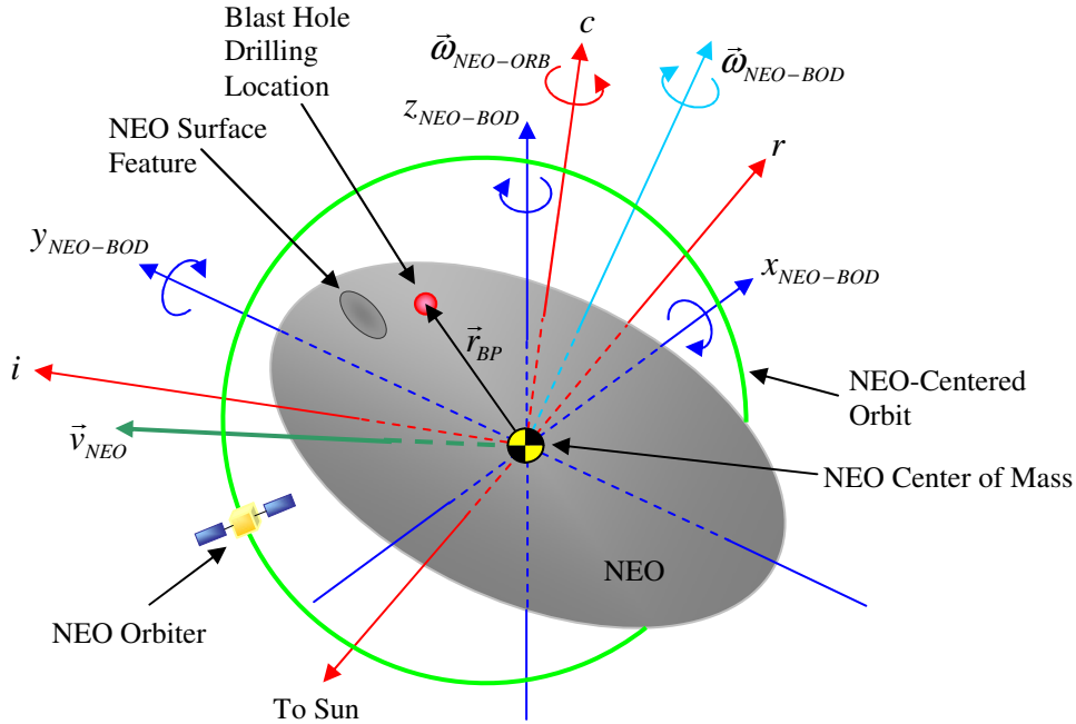
Figure 12. Reference frames and NEO-centered support spacecraft orbit required for proximity and surface operations.
