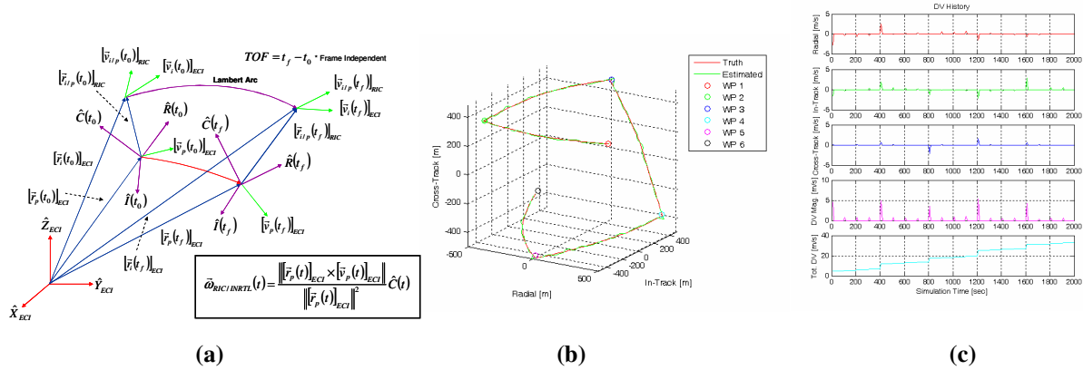
Figure 11. (a) Vector geometry for relative motion guidance using Lambert targeting, (b) relative motion achieved using Lambert relative guidance and applied control with navigation error in simulation, and (c) associated control history and fuel consumption in terms of \Delta v expenditure.
