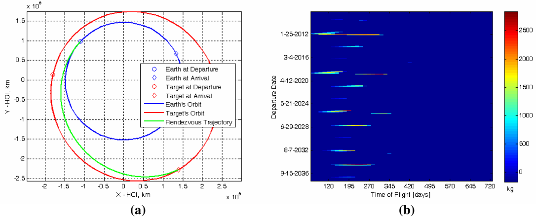
Figure 7. (a) Maximum Payload Mass Rendezvous with Asteroid Eros and (b) Maximum Payload Mass as a Function of Departure Date and Time of Flight
