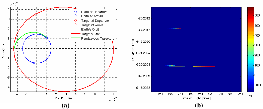
Figure 6. (a) Maximum Payload Mass Rendezvous with Comet 81P/Wild 2 and (b) Maximum Payload Mass as a Function of Departure Date and Time of Flight
