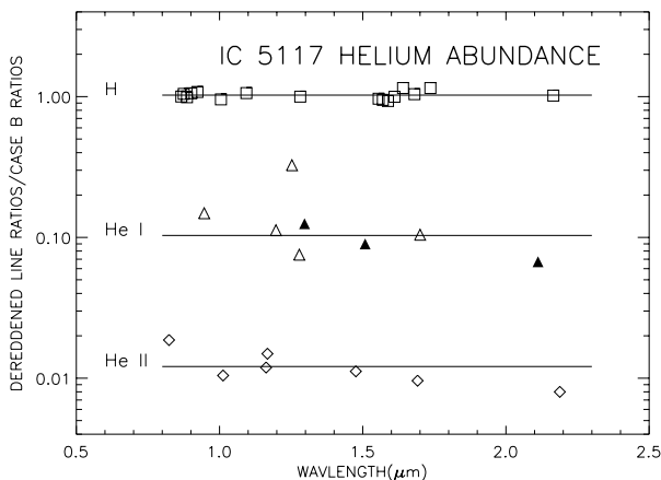
FIG. 4.—Helium-to-hydrogen abundance for IC 5117. The ordinate is the reddening-corrected flux ratio of the H, He I, or He II line, with respect to \text{Pa}\beta , divided by the case B value for the same ratio. Hydrogen lines are plotted as squares, He I as triangles (open for singlets, filled for triplets), and He II as diamonds. The individual lines can be identified from their wavelengths; for He I they are \lambda 9464, \lambda 11969, \lambda 12785, \lambda\lambda 12968, 12985, \lambda 17002, \text{ and } \lambda\lambda 21120, 21132 ( \lambda\lambda 12968 and 12985 have been combined, as have \lambda\lambda 21120 and 21132 ). He I \lambda 12528 is shown in the figure but was not used in the abundance determination, because of its well-known enhancement due to optical depth effects in \lambda 3188 (see text). The He II lines are \lambda 8237, \lambda 10124, \lambda 11626, \lambda 11673, \lambda 14760, \lambda 16915, \text{ and } \lambda 21882 . In this presentation, the relative abundance indicated by each line for its parent species can be read off of the y-axis. The horizontal lines indicate the average value for each of the species. The average relative abundances, by number, are \text{H}^+/\text{He}^+/\text{He}^{++} = 1.00/0.101/0.012 .
