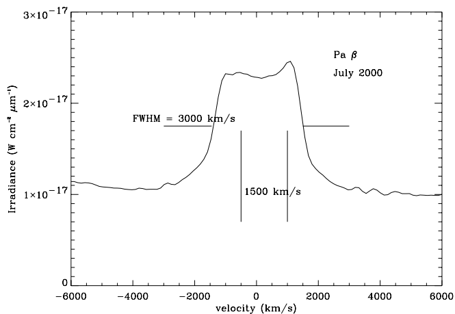
FIG. 4.—All of the line profiles show somewhat flattened top with evidence of doubling. Pa \beta is typical with a FWHM of about 3000 km s -1 and a splitting separation of around 1500 km s -1 . Lines of both high and low excitation are similar.
